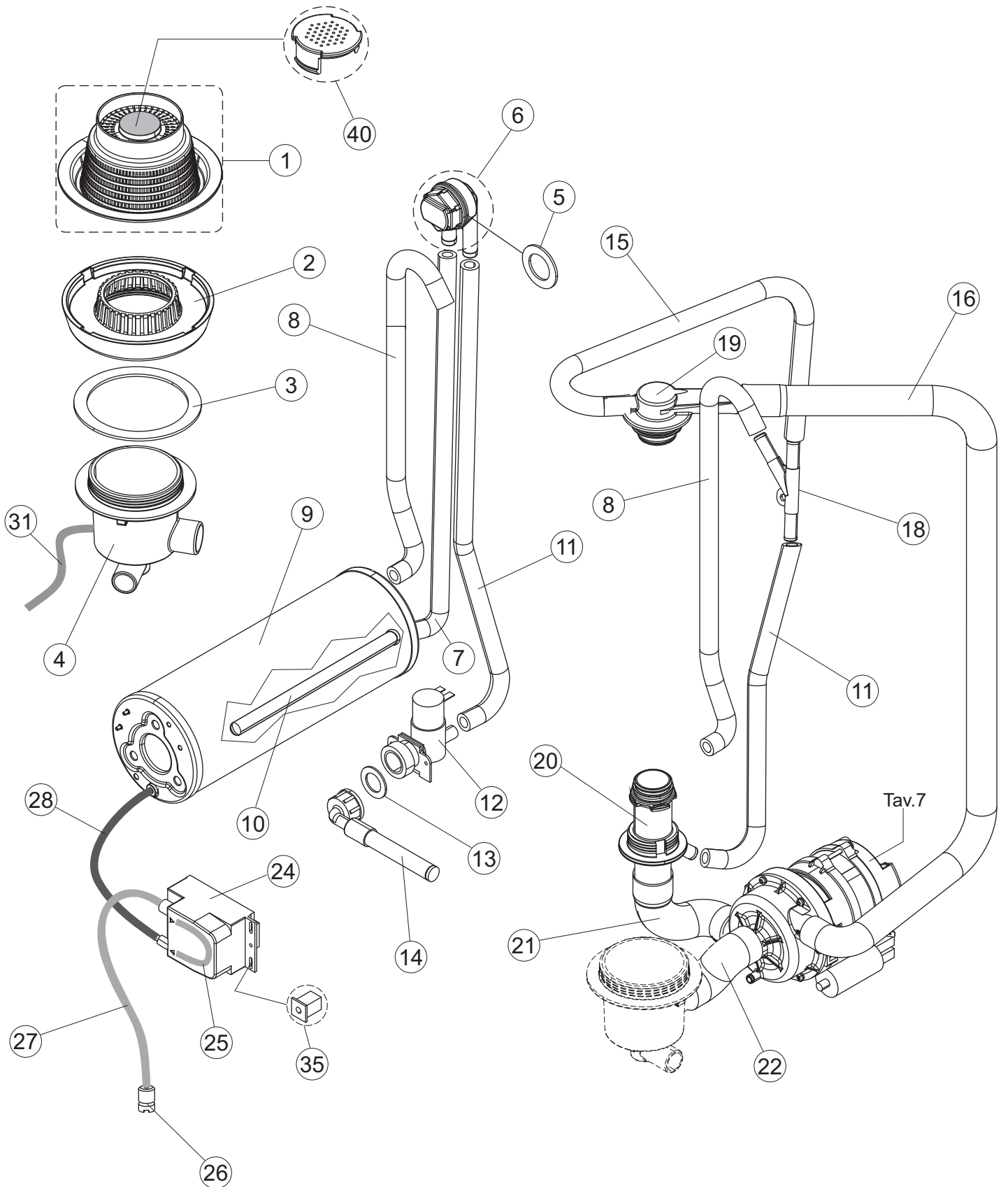
Drain Pump
